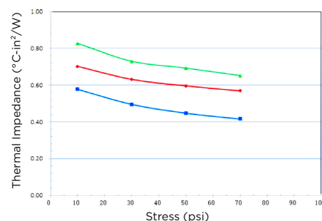
Thermal Impedance Vs. Stress of GP3100-H1/H0/HU (1.0mm thick) (@ Temp=60°C; Step application of pressure 10, 30, 50, 70 psi; ASTM D5470 modified)
