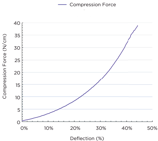
D Shape 1.0 mm(H) * 1.3 mm(W) Rate of Strain, 1.5mm/min Force-Deflection of F6003 Gasket
